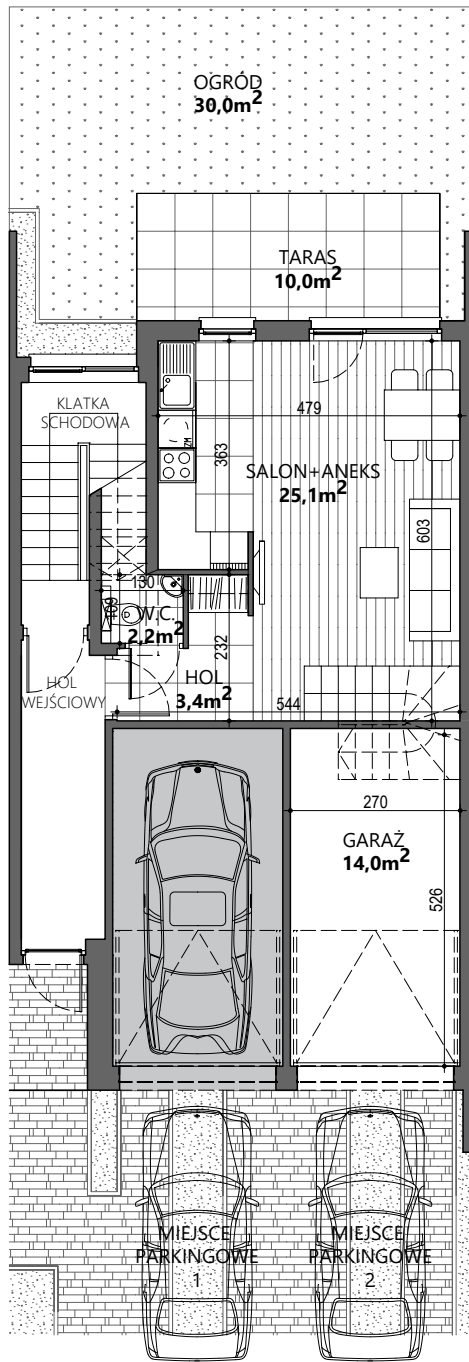
PARTER
